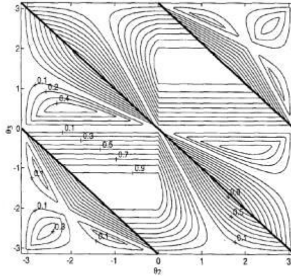
Figure 6: Contour of the minimum reduced manipulability index \mu(i_j) a RRR planar manipulator. The bold lines show configurations that optimal value for the minimum relative manipulability index [84]. (© [1996] IEEE) 7
